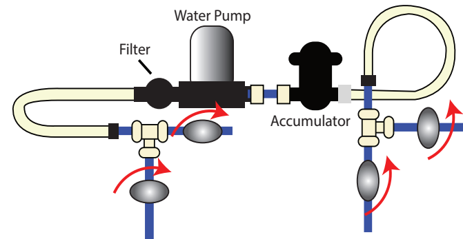
Boondocking Valve Configuration Drawing water from rear inlet to fill the fresh tank.
